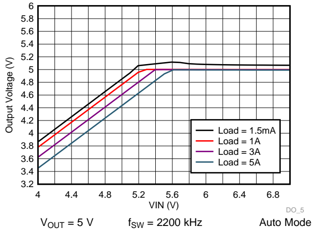
Figure 51. LM73605 Dropout Curve
