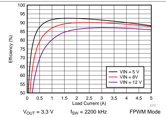
Figure 30. LM73605 Efficiency
