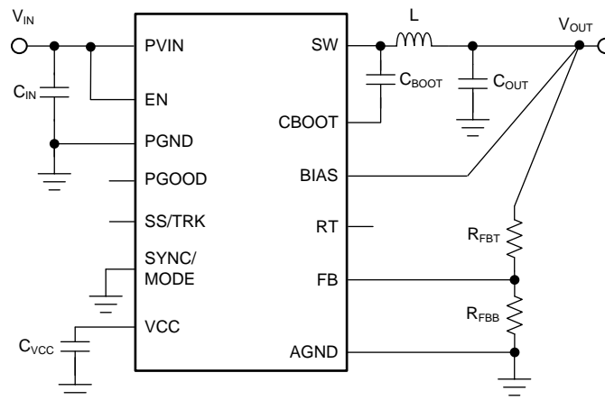
Figure 25. LM73605/6 Basic Schematic
