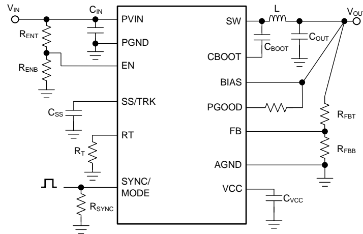
Figure 26. LM73605/6 Comprehensive Schematic with All Features Utilized
