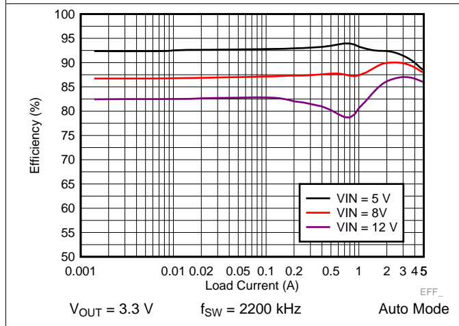
Figure 29. LM73605 Efficiency
