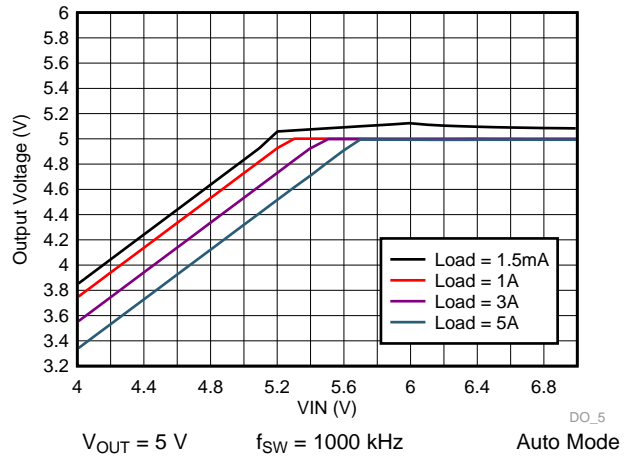
Figure 54. LM73605 Dropout Curve
