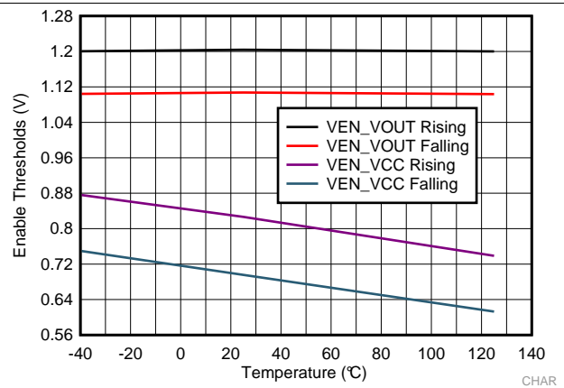
Figure 8. Enable Thresholds
