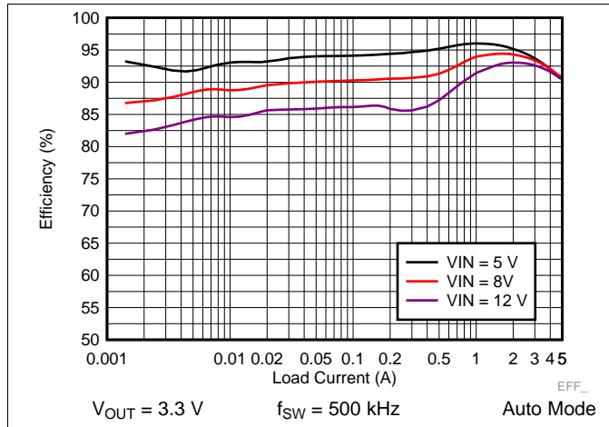
Figure 27. LM73605 Efficiency
