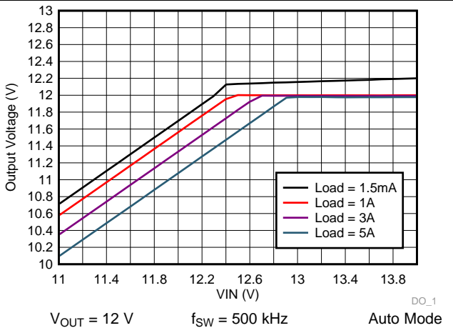
Figure 56. LM73605 Dropout Curve
