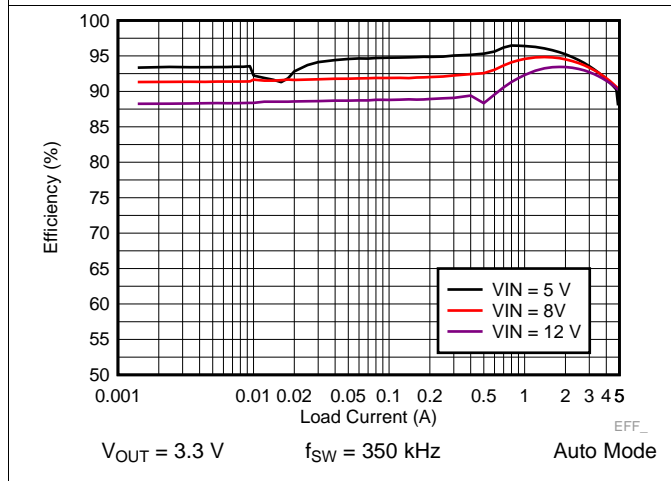
Figure 31. LM73605 Efficiency
