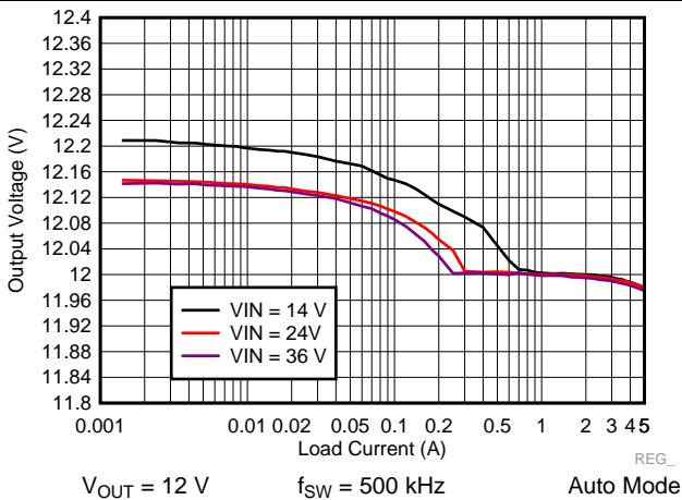
Figure 49. LM73605 Load and Line Regulation
