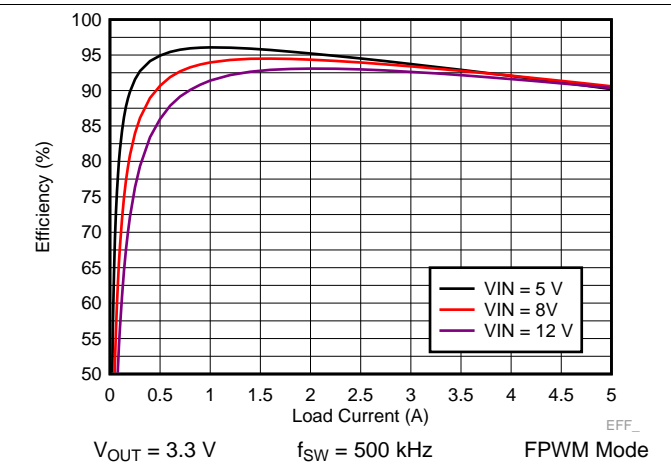
Figure 28. LM73605 Efficiency
