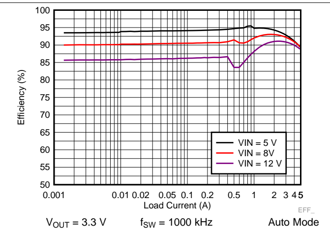
Figure 32. LM73605 Efficiency
