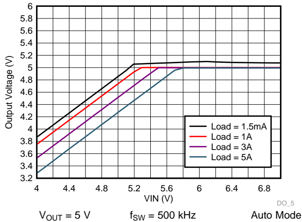
Figure 53. LM73605 Dropout Curve
