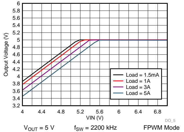
Figure 52. LM73605 Dropout Curve
