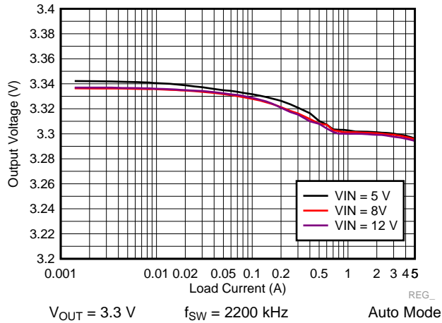
Figure 45. LM73605 Load and Line Regulation
