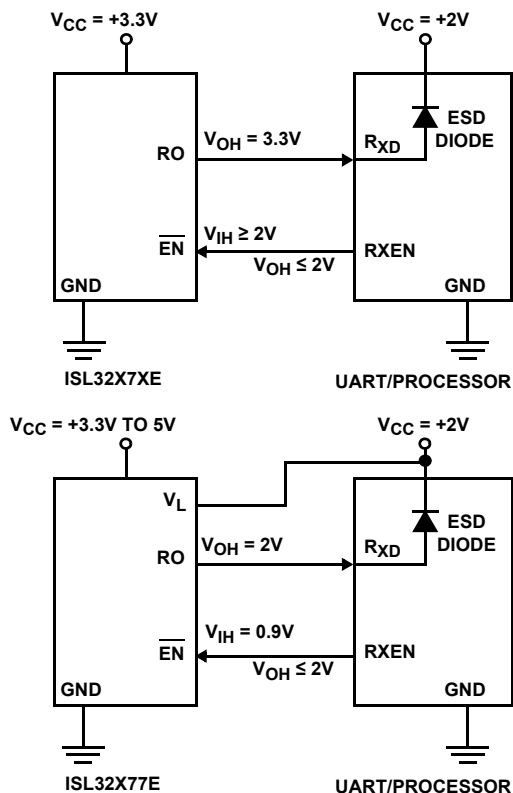
FIGURE 9. USING V_{\text{L}} PIN TO ADJUST LOGIC LEVELS
