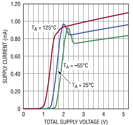
Supply Current vs Supply Voltage (Per Amplifier)
