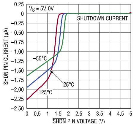
SHDN Pin Current vs SHDN Pin Voltage
