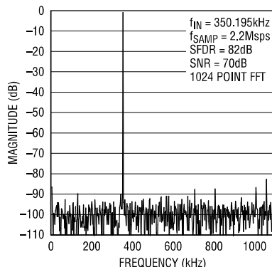
350kHz FFT Driving ADC
