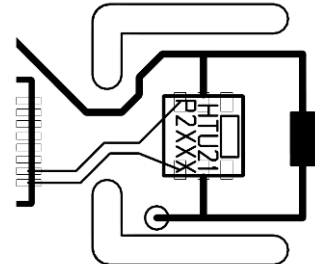
Example of HTU21P(F) sensor mounting with slits mills to minimize heat transfer
