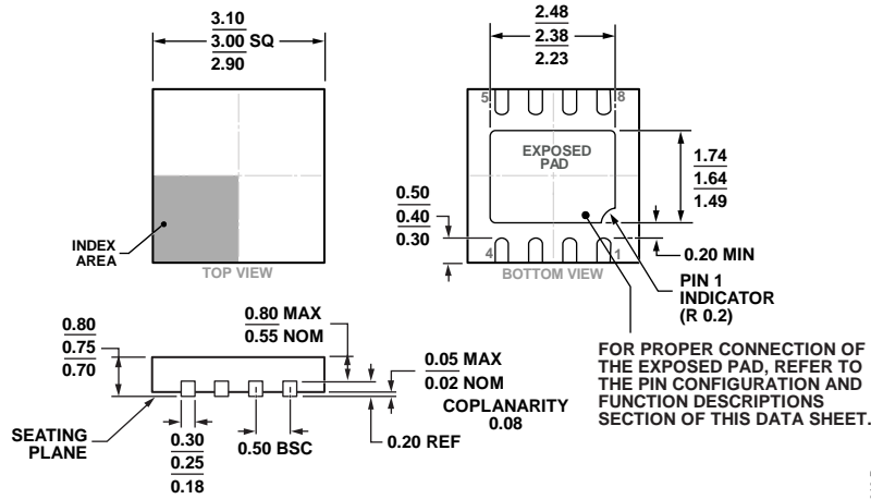
Figure 80. 8-Lead Lead Frame Chip Scale Package [LFCSP_WD] 3 mm x 3 mm Body, Very Very Thin, Dual Lead (CP-8-5)
