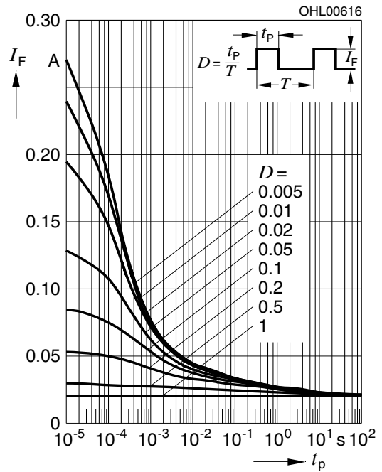
Zulässige Impulsbelastbarkeit I_F = f(t_p) Permissible Pulse Handling Capability Duty cycle D = parameter, T_A = 85\text{ °C} LO, LY
