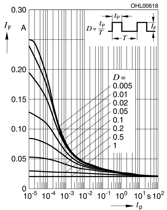
Zulässige Impulsbelastbarkeit I_F = f(t_p) Permissible Pulse Handling Capability Duty cycle D = parameter, T_A = 85\text{ °C} LO, LY
