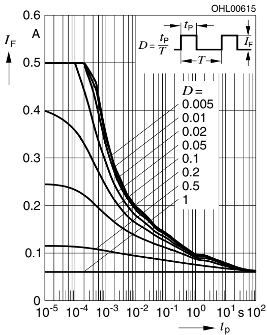
Zulässige Impulsbelastbarkeit I_F = f(t_p) Permissible Pulse Handling Capability Duty cycle D = parameter, T_A = 25\text{ °C} LO, LY
