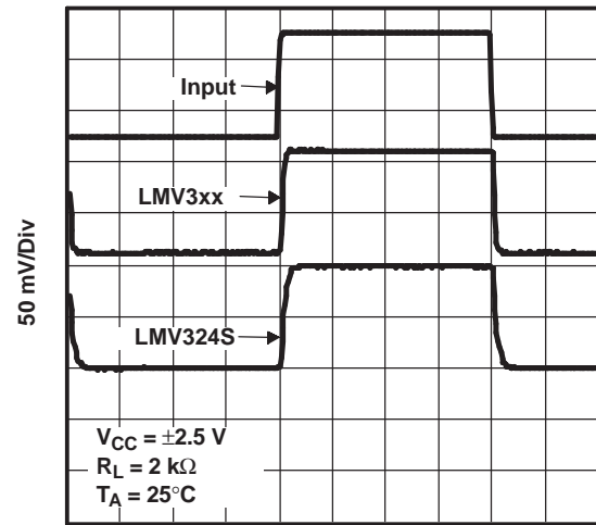
1 \mu\text{s}/\text{Div} Figure 30.
