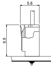
PA Receptacle (Standard type) + PA Header
