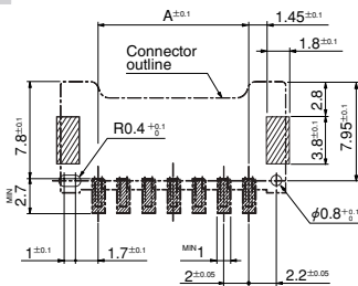
PA Receptacle (Standard type) + PA side entry type header
