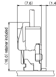
PA Receptacle (Retainer mountable type) + PA Header
