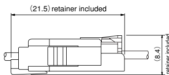
PA Receptacle (Standard type) + PAL Receptacle
