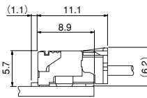
PA Receptacle (Standard type) + PA side entry type header
