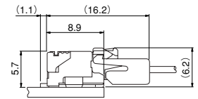
PAF Receptacle + PA side entry type header
