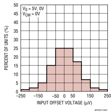
V_{OS} Distribution, V_{CM} = 0\text{V} (S8, PNP Stage)
