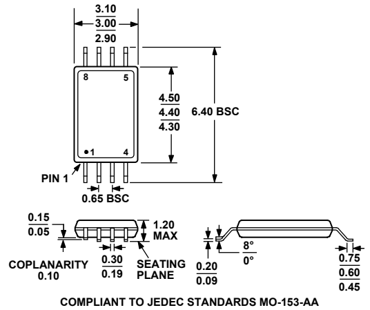
COMPLIANT TO JEDEC STANDARDS MO-153-AA Figure 71. 8-Lead Thin Shrink Small Outline Package [TSSOP] (RU-8) Dimensions shown in millimeters
