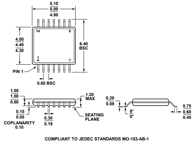
COMPLIANT TO JEDEC STANDARDS MO-153-AB-1 Figure 72. 14-Lead Thin Shrink Small Outline Package [TSSOP] (RU-14) Dimensions shown in millimeters
