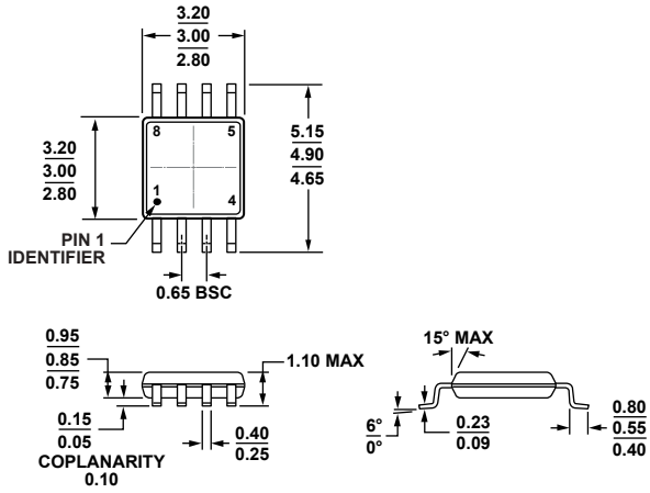
COMPLIANT TO JEDEC STANDARDS MO-187-AA Figure 69. 8-Lead Mini Small Outline Package [MSOP] (RM-8) Dimensions shown in millimeters
