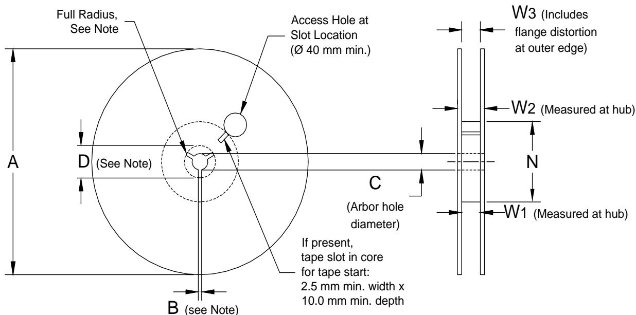
Figure 5 – Reel Dimensions
