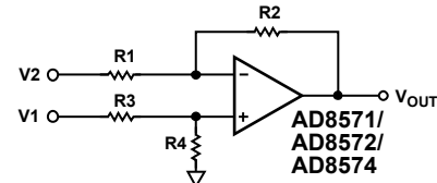
Figure 64. Using the AD857x as a Difference Amplifier
