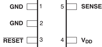
TPS3801-01 . . . DCK PACKAGE (TOP VIEW)
