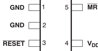
TPS380x . . . DCK PACKAGE (TOP VIEW)
