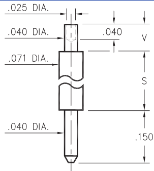
312X-X-00-XX-00-00-08-0 Swage mount in .043 hole
