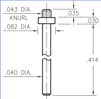
4526-0-00-XX-00-00-03-0 Press-fit in .040 mounting hole
