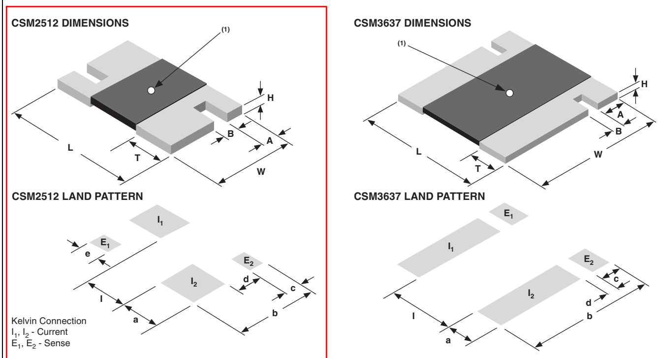
FIGURE 2 - DIMENSIONS AND IMPRINTING in inches (millimeters)
