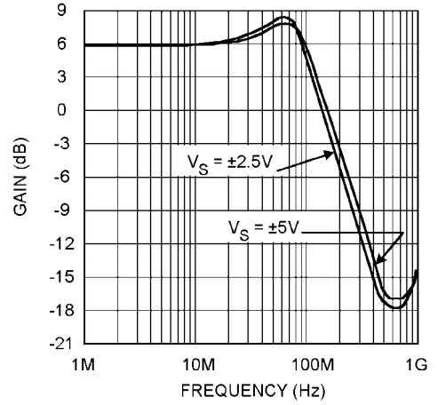
Closed Loop Bandwidth (G = +2)
