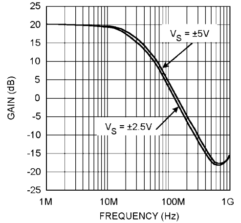
Closed Loop Bandwidth (G = +10)
