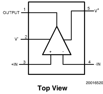
5-Pin SOT-23 (LMH6654)
