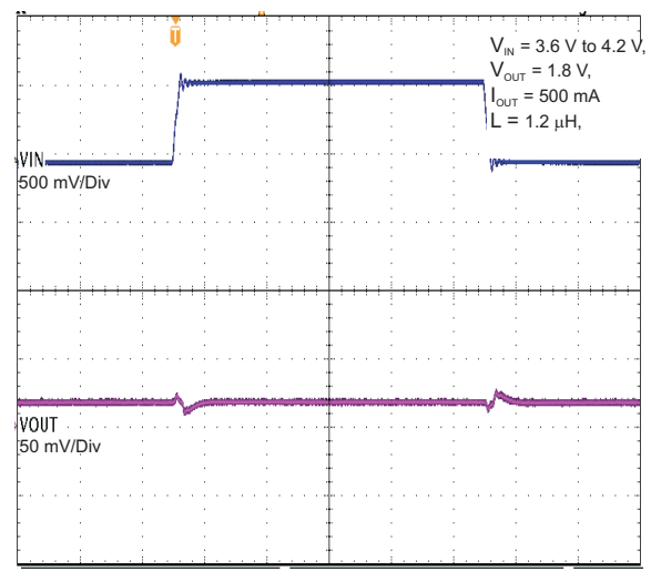
Time Base - 100 \mu s/Div
