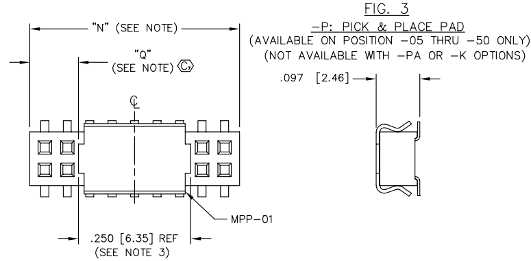
FIG. 3 -P: PICK & PLACE PAD (AVAILABLE ON POSITION -05 THRU -50 ONLY) (NOT AVAILABLE WITH -PA OR -K OPTIONS) AVAILABLE ON POSITIONS 05 THRU 50 ONLY NOTE: "N" = USED MEASURED DIMENSION (REF) "Q" = {"N" - .250 [6.35]} / 2 ± .020 [.51]
