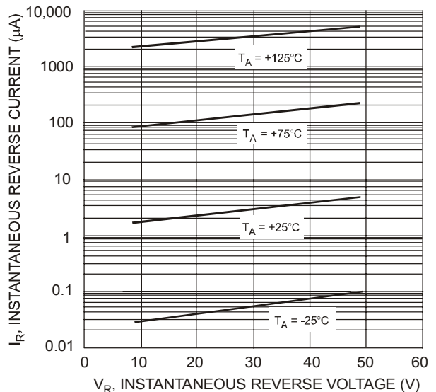
Fig. 6 Typical Reverse Characteristics, B320A thru B340A
