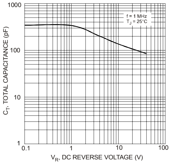
Fig. 5 Typical Capacitance
